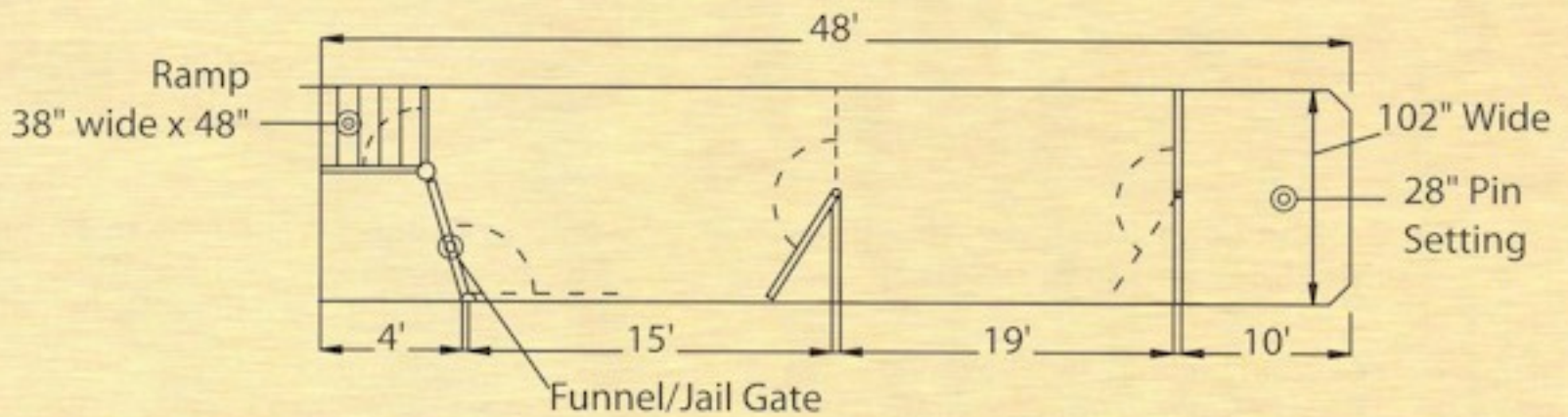
Interior Layout for Standard 48' Groundload
